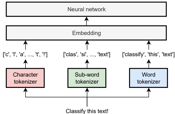
Figure 3: Character, subword and word tokenization. Subword tokenizers learn reusable pieces from a corpus, for example with byte pair encoding (BPE).
