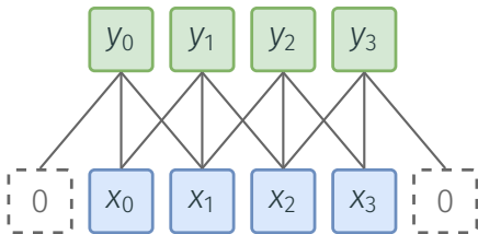
Stride 1: four outputs
