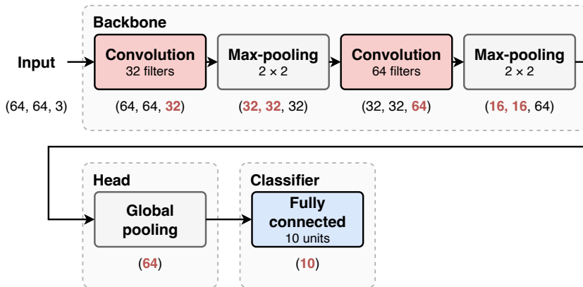
Figure 1: Down-sampling reduces the cost of subsequent layers. Global pooling makes the final classification dimensionality manageable.
