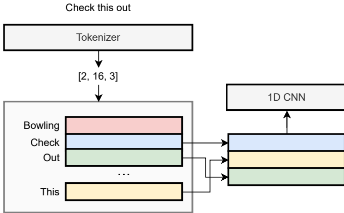
Figure 4: Using custom embeddings for text classification.
