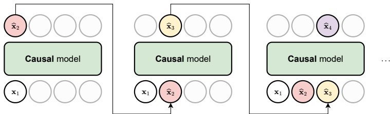
Figure 5: The hat marks a generated value: \hat{x}_{t+1} is the model's prediction for position t + 1 , which is fed back as the next input. For text, we feed back sampled token IDs. Gray circles mark unused positions.
