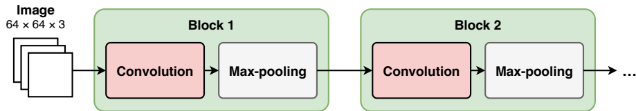
Figure 2: When CNNs become deep, it is simpler to reason in repeating blocks made of multiple components. This is easy using the layering abstraction.
